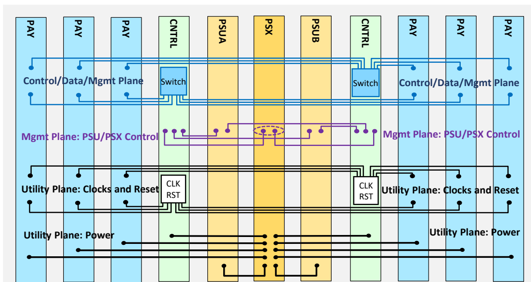
Figure 2: SpaceVPX Backplane with Combined Control, Data and Payload Management Plane
