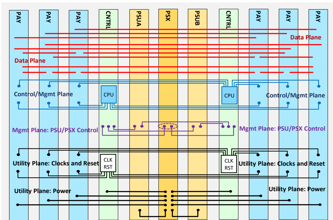
Figure 1: SpaceVPX-Lite Backplane with Combined Control/Management Plane to the Payload Modules
