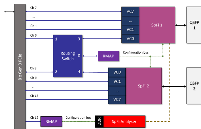
STAR-Ultra PCIe Functional Block Diagram
