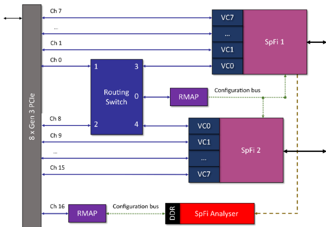
STAR-Ultra PCIe Functional Block Diagram
