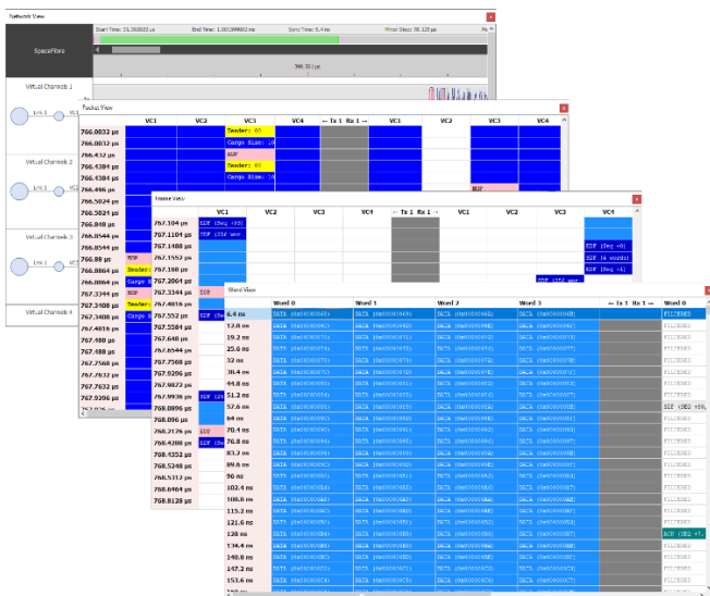
STAR-Ultra PCIe Link Analyser Views
