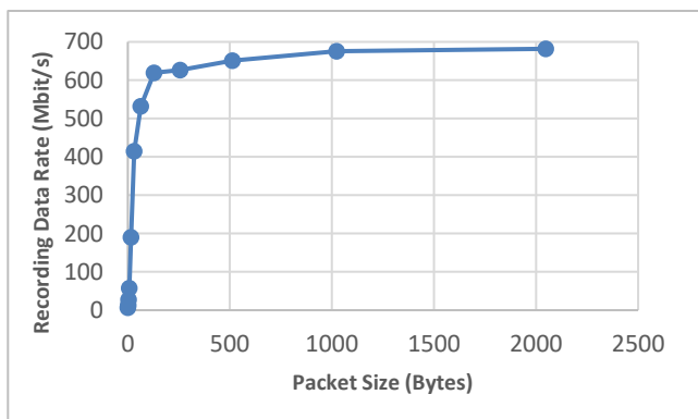
Packet Size vs Aggregate Recording Data Rate
